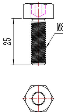
② Dual Hex Bolt (M8-25mm)
